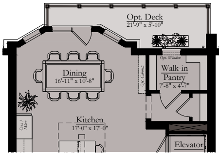
Opt. Main Level Deck - Elevations A & B
