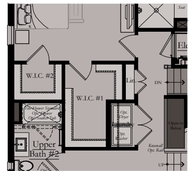
Opt. Owner's Enlarged Walk-In Closet
