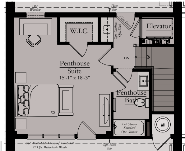
Opt. Penthouse Suite - Elevations A, B, & C
