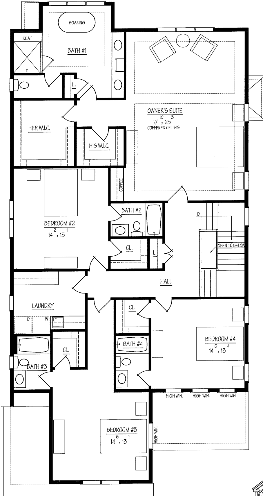
SECOND FLOOR PLAN 2195 SQ. FT. MAIN RENDERING ONLY: DIMENSIONS MAY VARY
