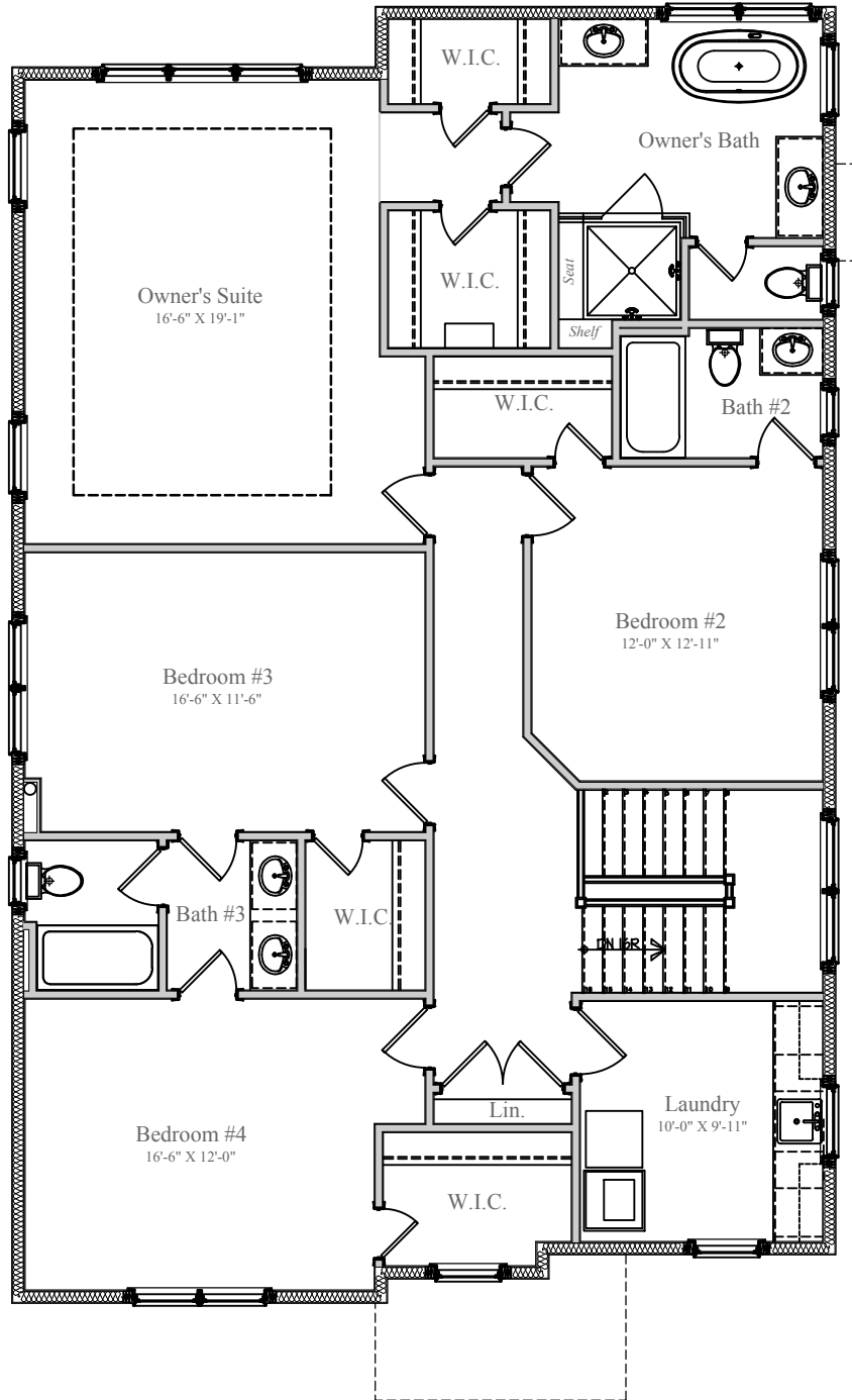
UPPER LEVEL FINISHED AREA: 2,066 sq. ft. DIMENSIONS MAY VARY
