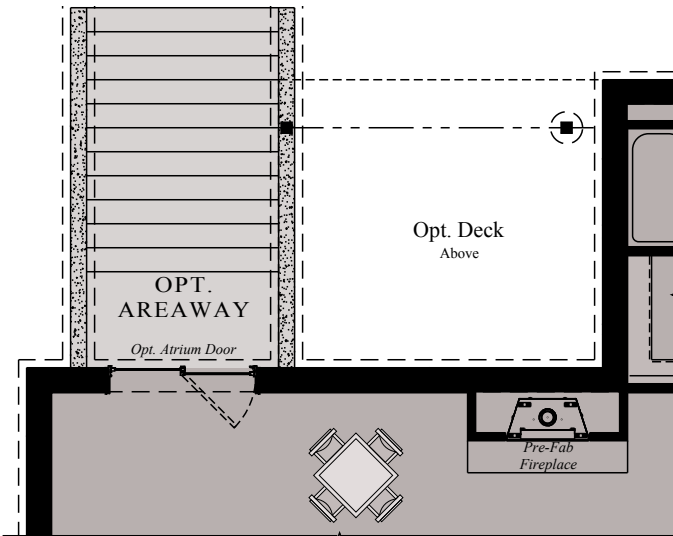
PARTIAL LOWER LEVEL - OPTIONAL 5' EXTENSION W/ OPTIONAL AREAWAY
