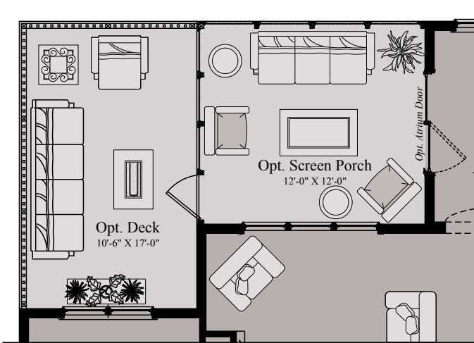
PARTIAL MAIN LEVEL - OPTIONAL SCREEN PORCH
