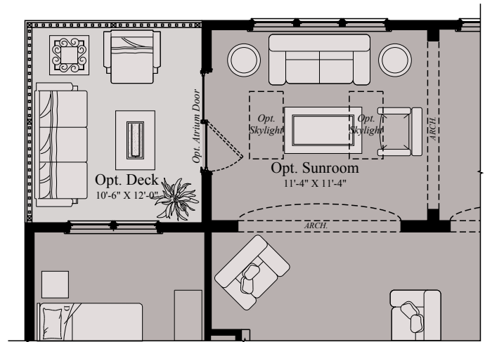
PARTIAL MAIN LEVEL - OPTIONAL SUNROOM W/ 5' EXTENSION
