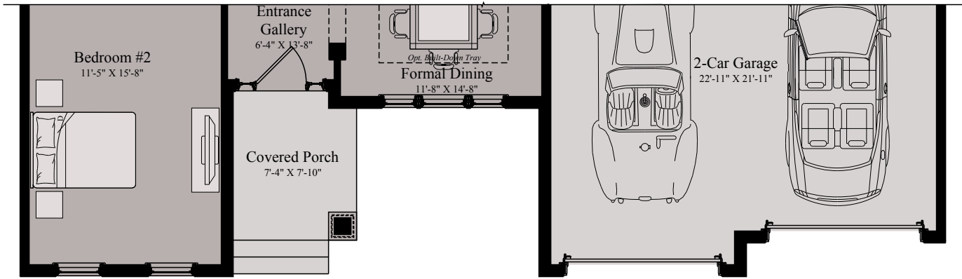
PARTIAL MAIN LEVEL - ELEVATION B
