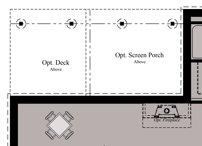
PARTIAL LOWER LEVEL - W/ OPTIONAL DECK OPTIONAL SCREENED PORCH OPTIONAL 5' EXTENSION
