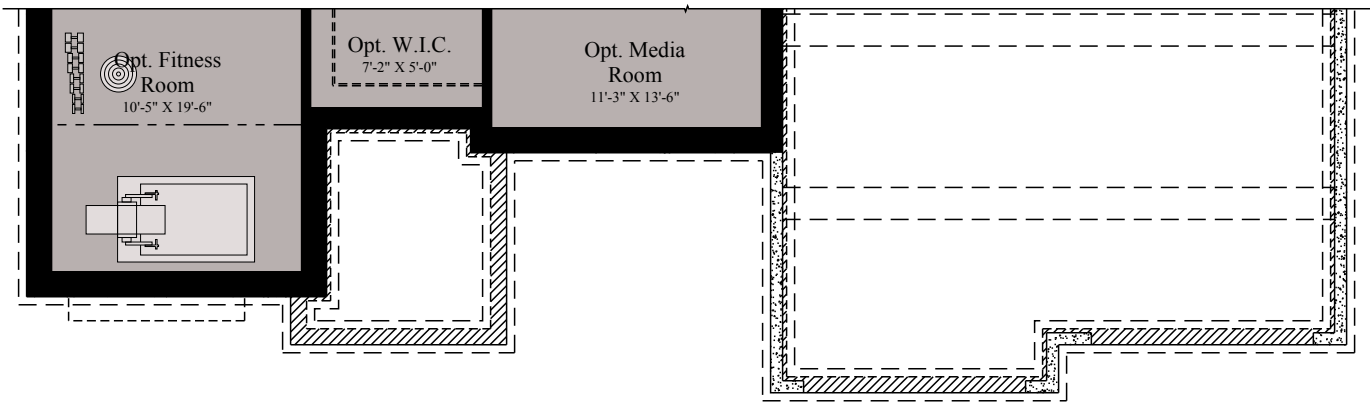
PARTIAL LOWER LEVEL - ELEVATION C
