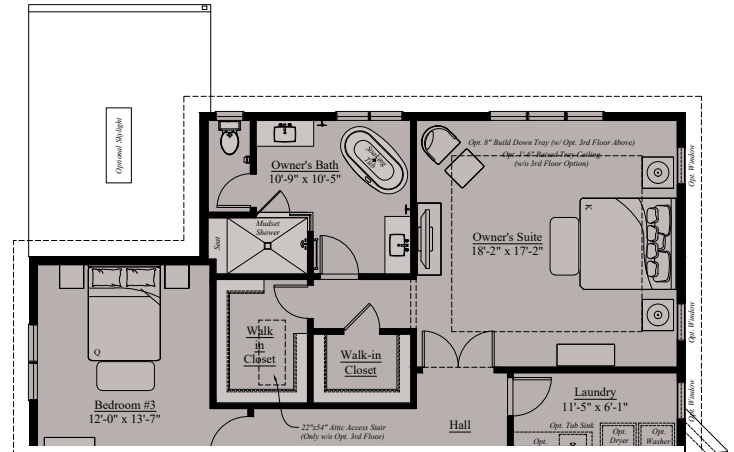
Second Floor w/ Optional Covered Deck or Sunroom
