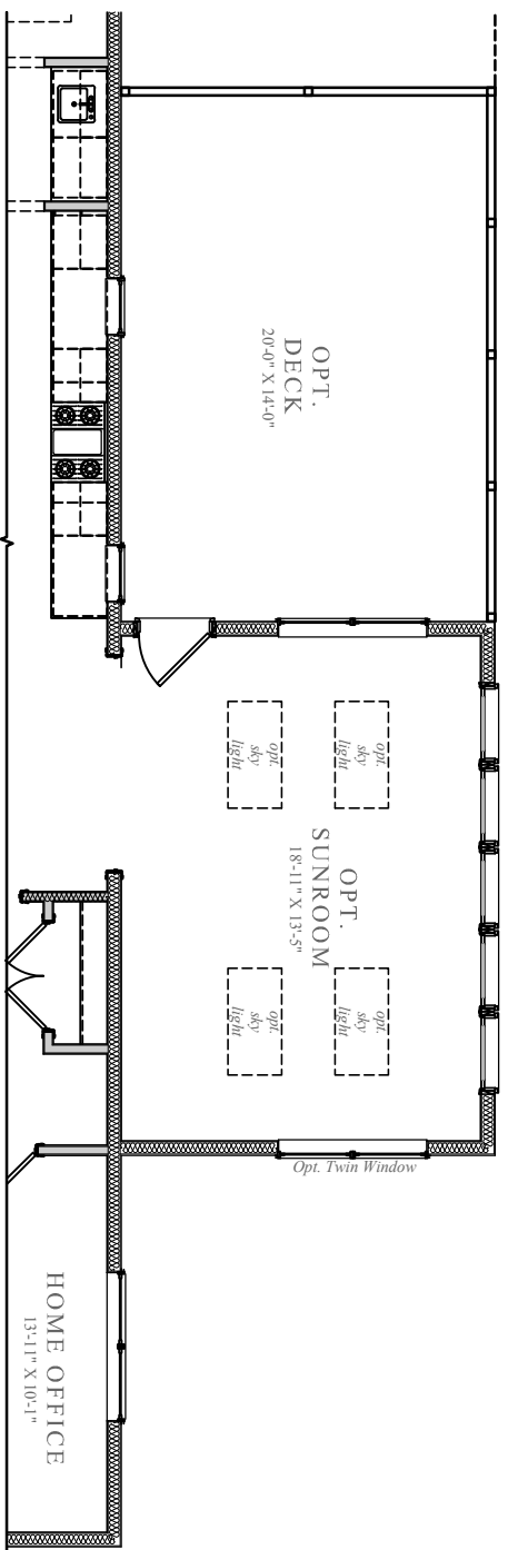
Partial Main Level Plan w/ Optional Sunroom
