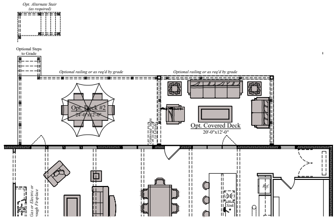
OPT. COVERED PORCH w/ OPT. DECK #2
