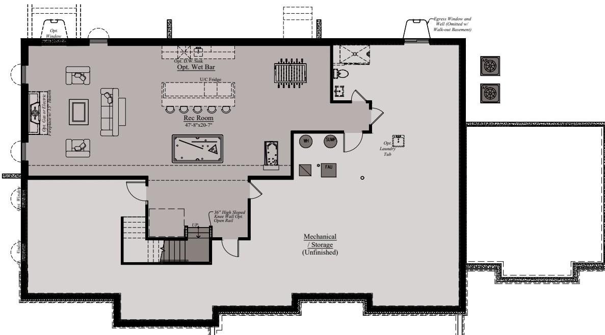
FINISHED REC ROOM
