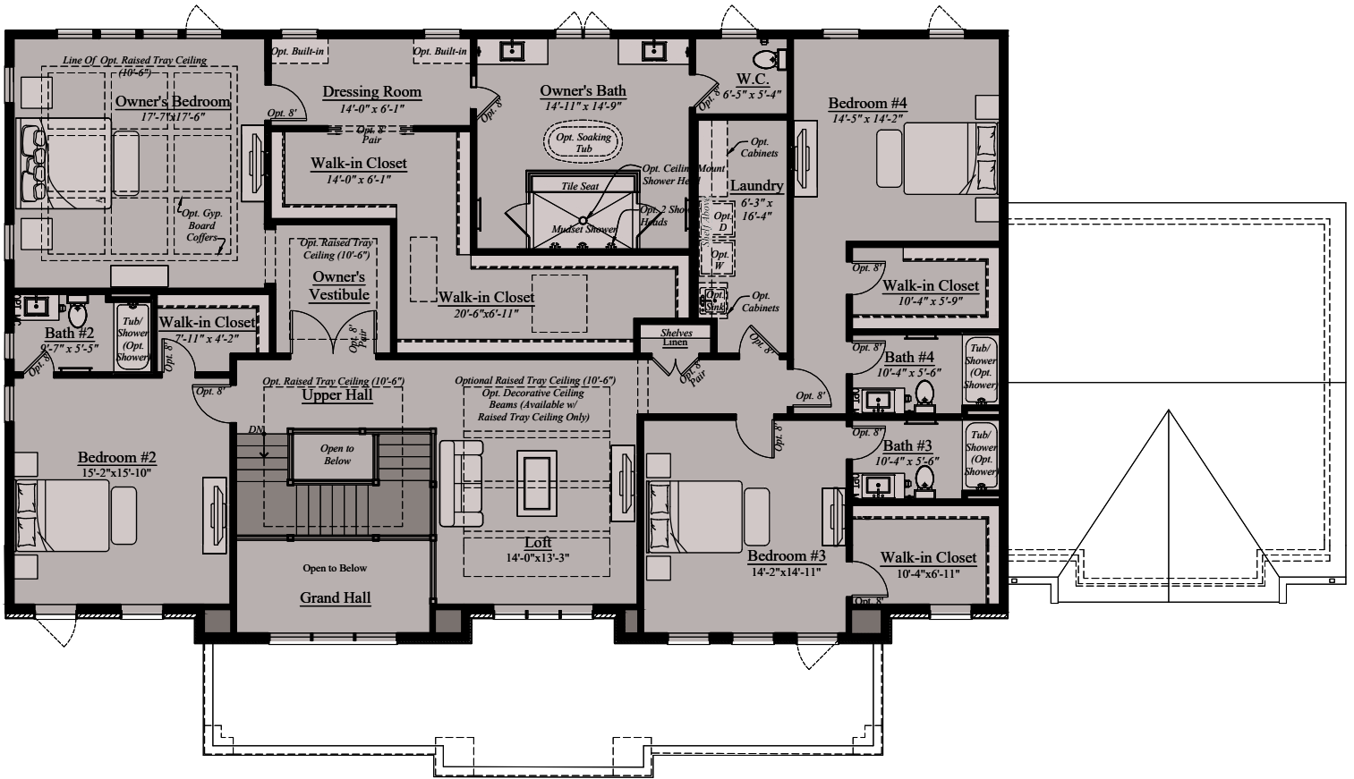
UPPER LEVEL 'A'
