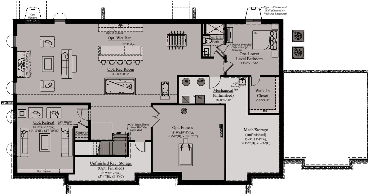
OPT. FINISHED LOWER LEVEL
