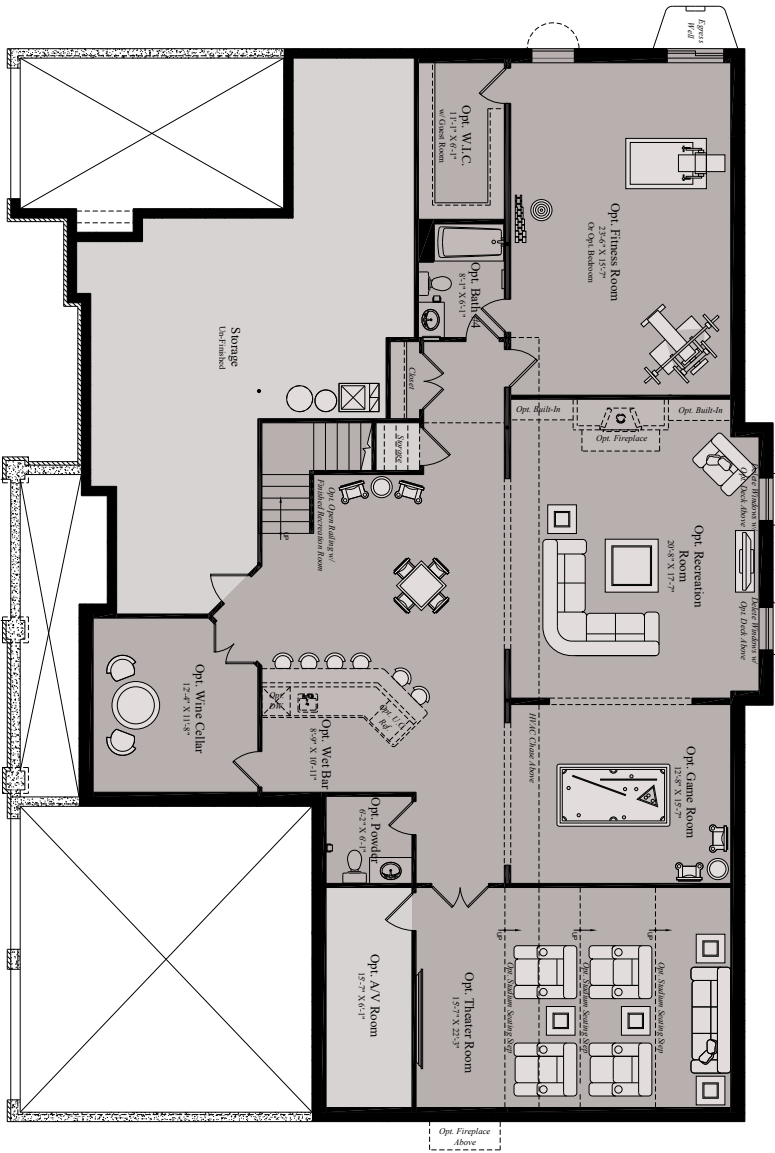
IN-GROUND CONDITION FINISHED LOWER LEVEL PLAN - ELEVATION "A"
