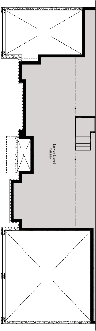
PARTIAL UNFINISHED LOWER LEVEL PLAN - ELEVATION "C"
