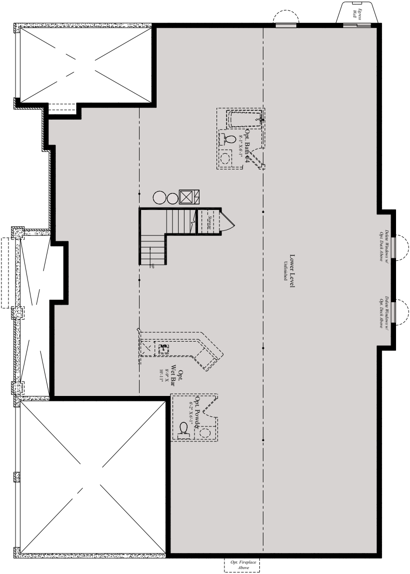
IN-GROUND CONDITION - UNFINISHED LOWER LEVEL PLAN - ELEVATION "A"
