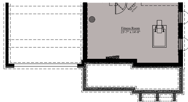
Elevation C - Lower Level
