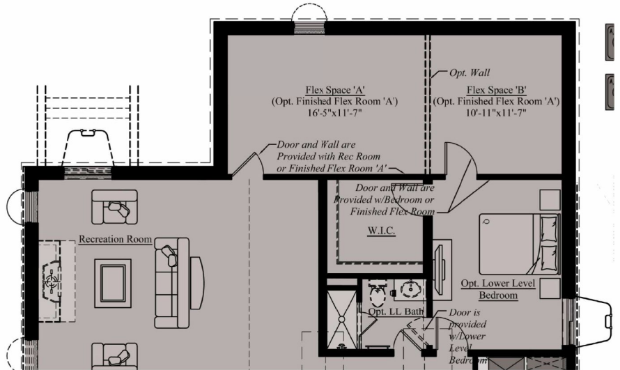
Opt. Flex Room A and B w/ Opt Lower Level Bedroom
