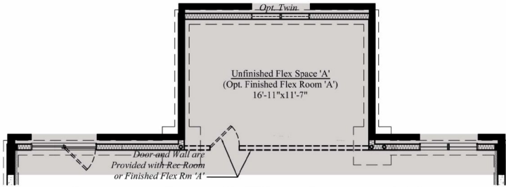
Lower Level Flex Room 'A' Walk-Out Condition
