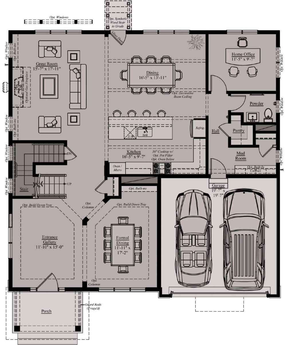
Main Level 'A'
