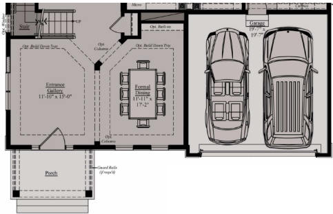
Main Level 'B'
