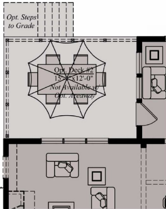
Opt. Deck #2 w/ Opt. Sunroom
