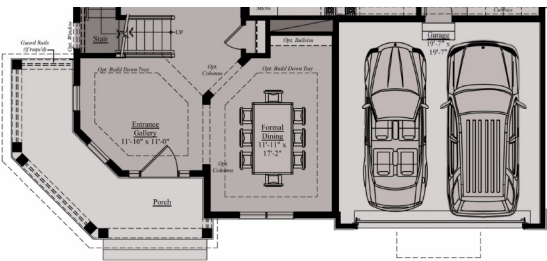
Main Level 'D'
