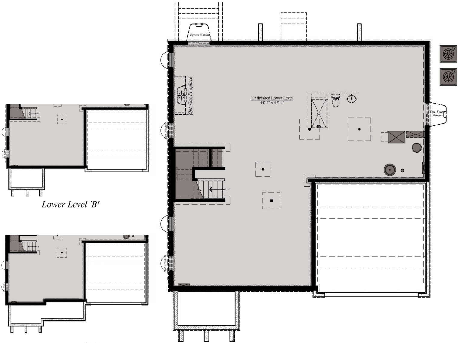
Lower Level 'C'
