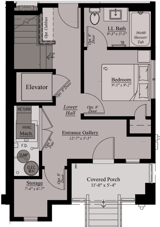
Opt. Bedroom at Lower Level (Available at End Units Only)
