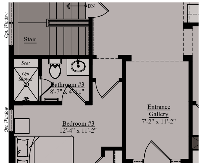
Opt. Bathroom #3
