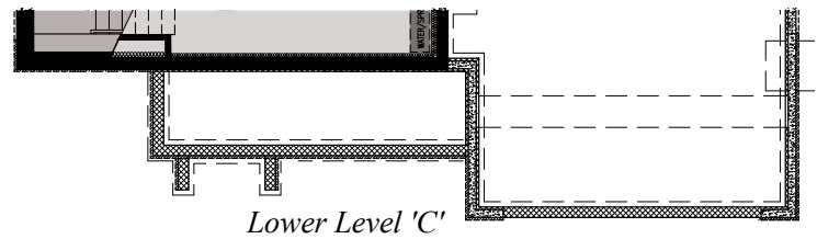
Finished Basement Plan
