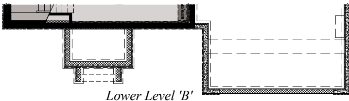
Finished Basement Plan
