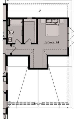
Opt. 3-Car Garage Elev 'B' - Upper Level
