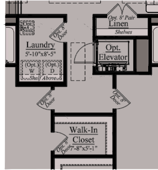
Opt. Elevator Upper Level
